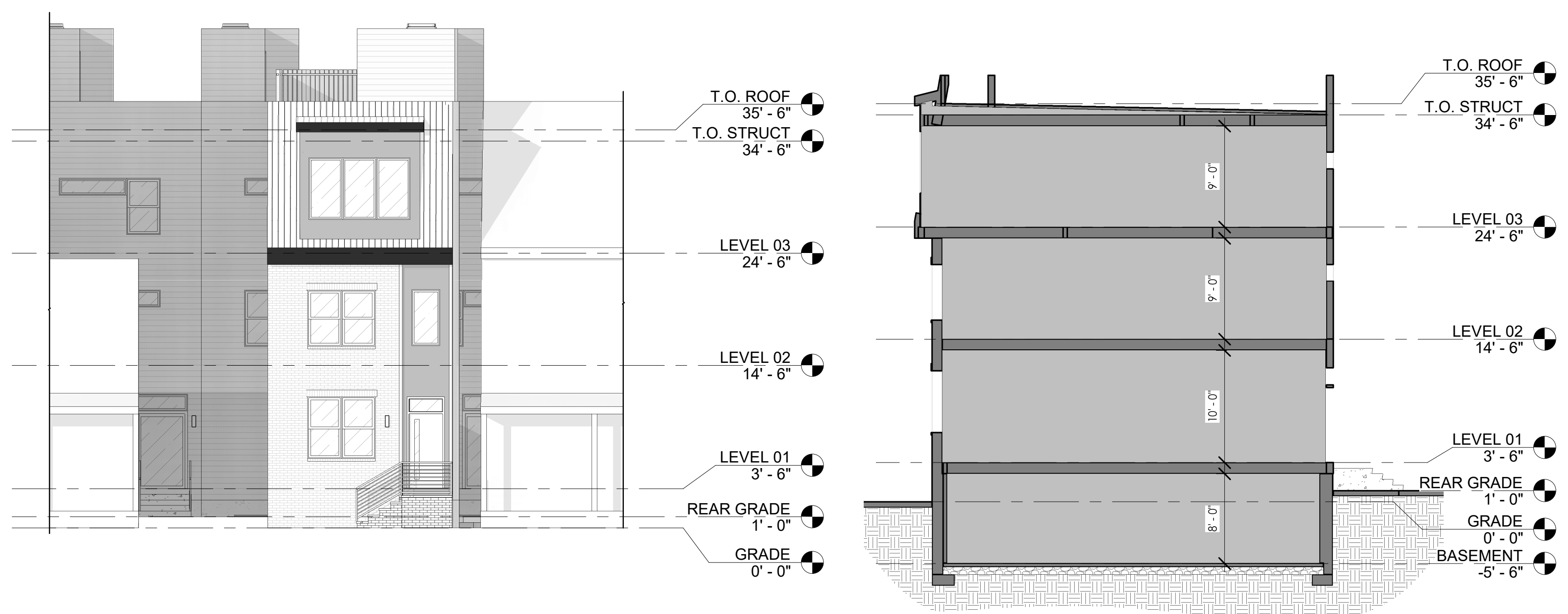
MEEHAN ST FRONT ELEVATION
